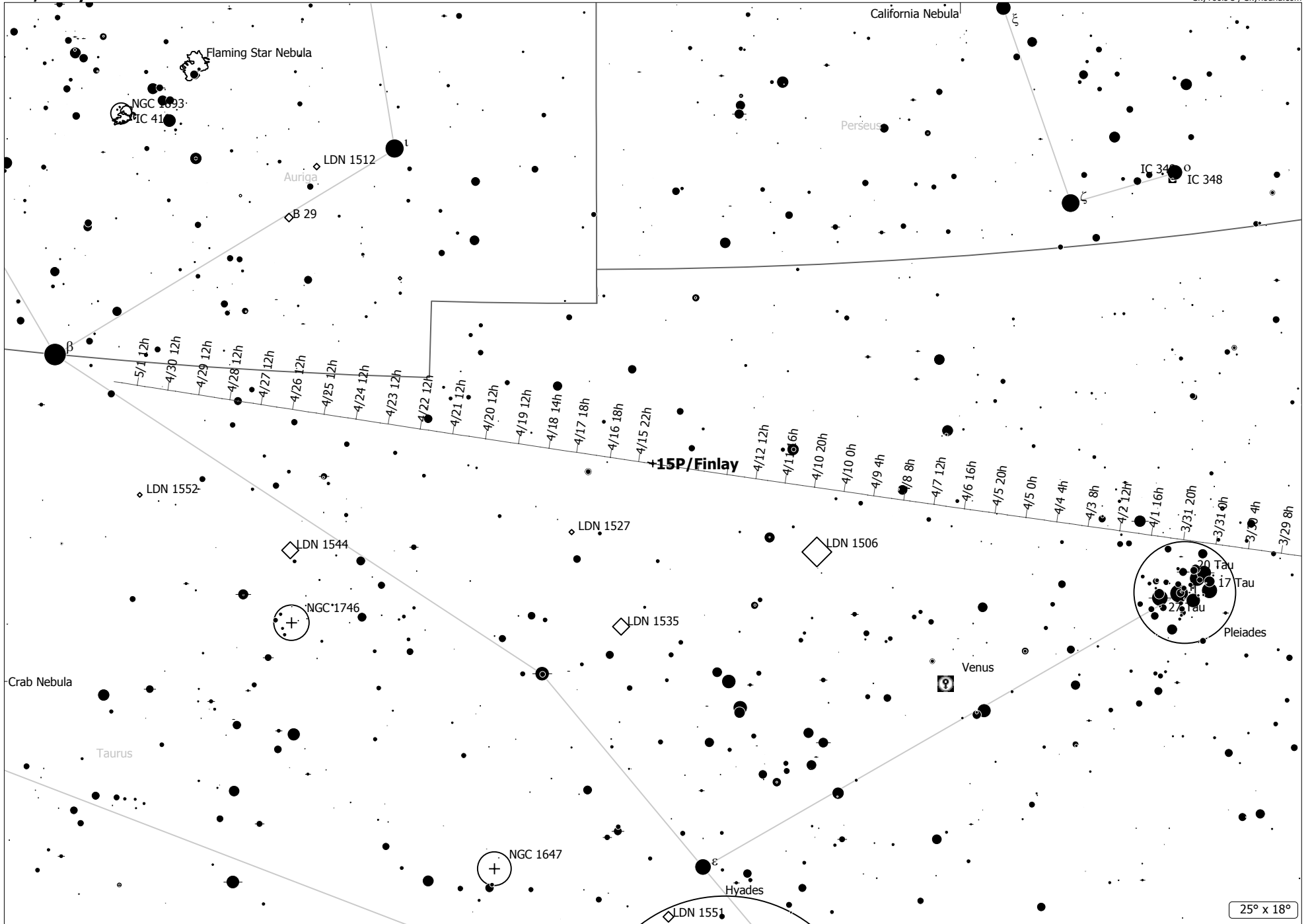
15P/Finlay (Comet)
