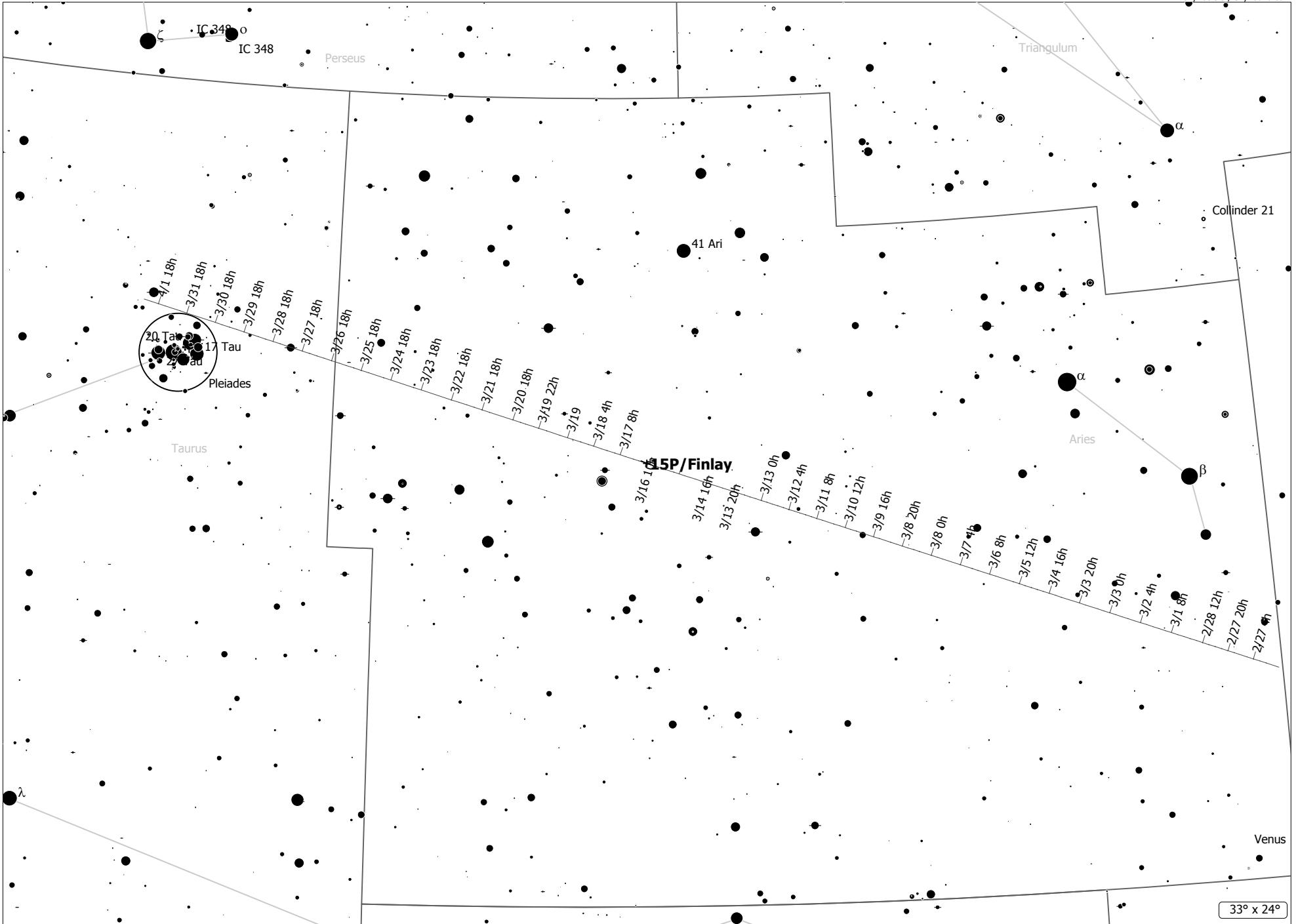
15P/Finlay (Comet)
