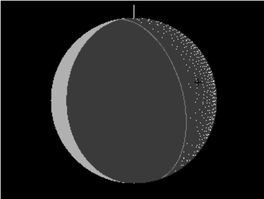
LEO Nov 17, 2006 17:47 UT -0.9 hrs Moon rises 2.4 hrs before sunrise zhr = 100 20% impacts on unlit near side w/polar graze = 10 deg
