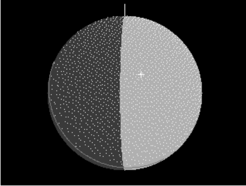
AUR Sep 1, 2006 06:05 UT +1.5 hrs Moon sets 6.2 hrs after sunset zhr = 10 36% impacts on unlit near side w/polar graze = 20 deg
